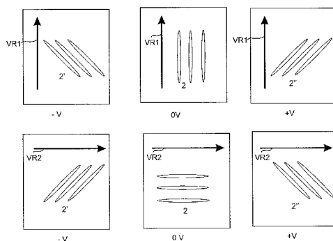
PSS with switchable surface orientation (VR1 > VR2) and all up 180° settable turning angle of the LC molecules 2
