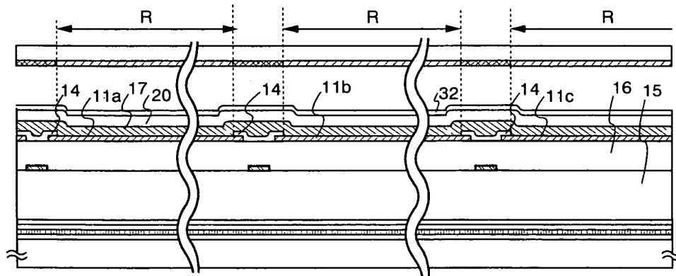
FIG. 1B sectional view of B-B'
