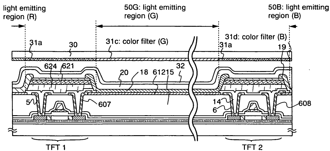
FIG. 6B sectional view of B-B'
