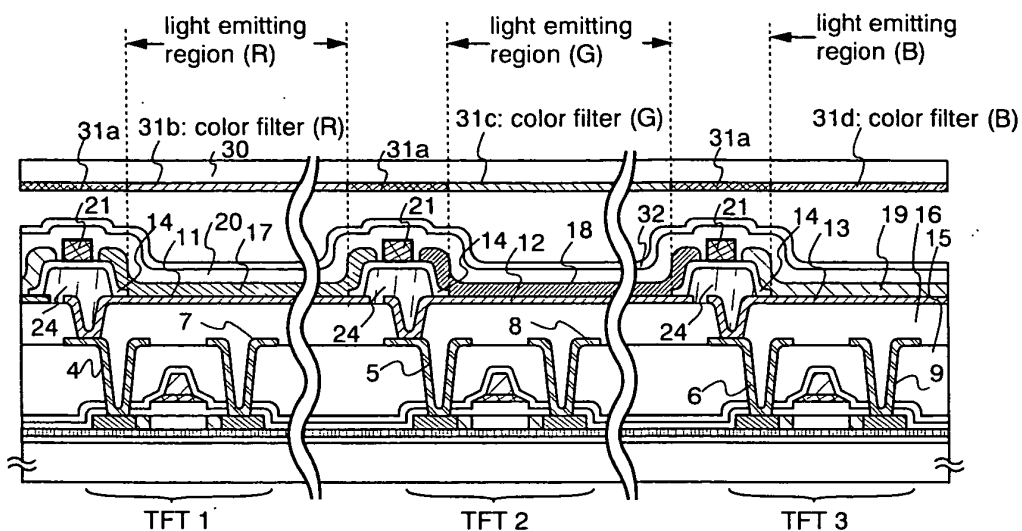
FIG. 1B sectional view of B-B'
