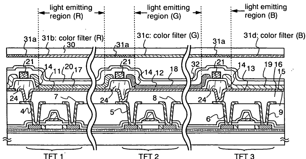
FIG. 1A sectional view of A-A'
