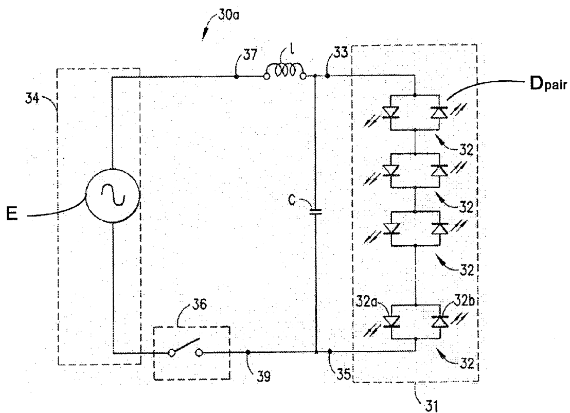
FIG. 3(Prior Art)
