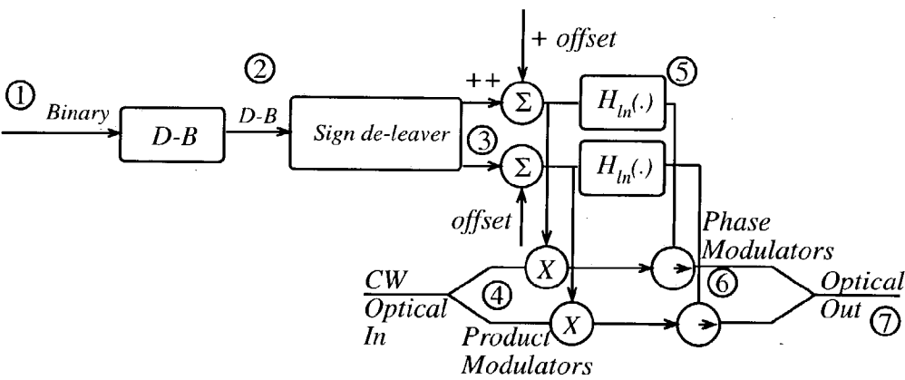
Figure 2. Duo-binary (Polybinary) Envelope Compatible Single Sideband Modulator
