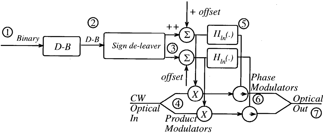
Duo-binary (Polybinary) Envelope Compatible Single Sideband Modulator
