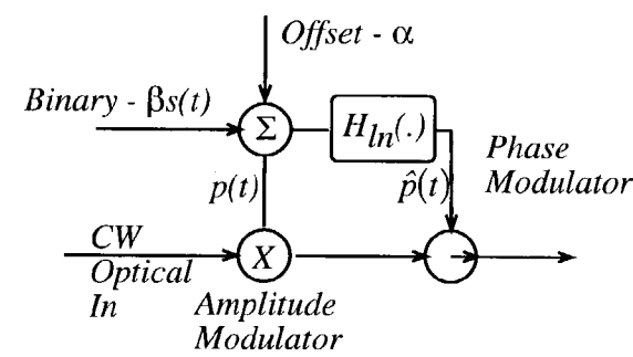
Figure 1. Minimum Phase SSB Modulator
