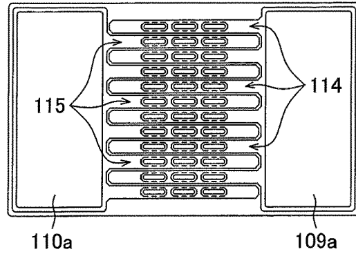
FIG. 22E Arrangement Example 105
