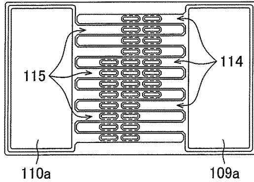
FIG. 22F Arrangement Example 106
