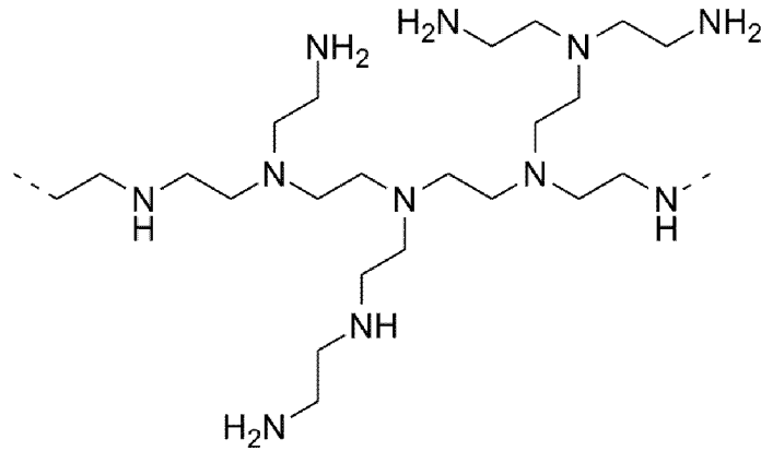
Exemplary Branched PEI
