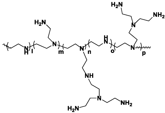
Branched Polyethyleneimine
