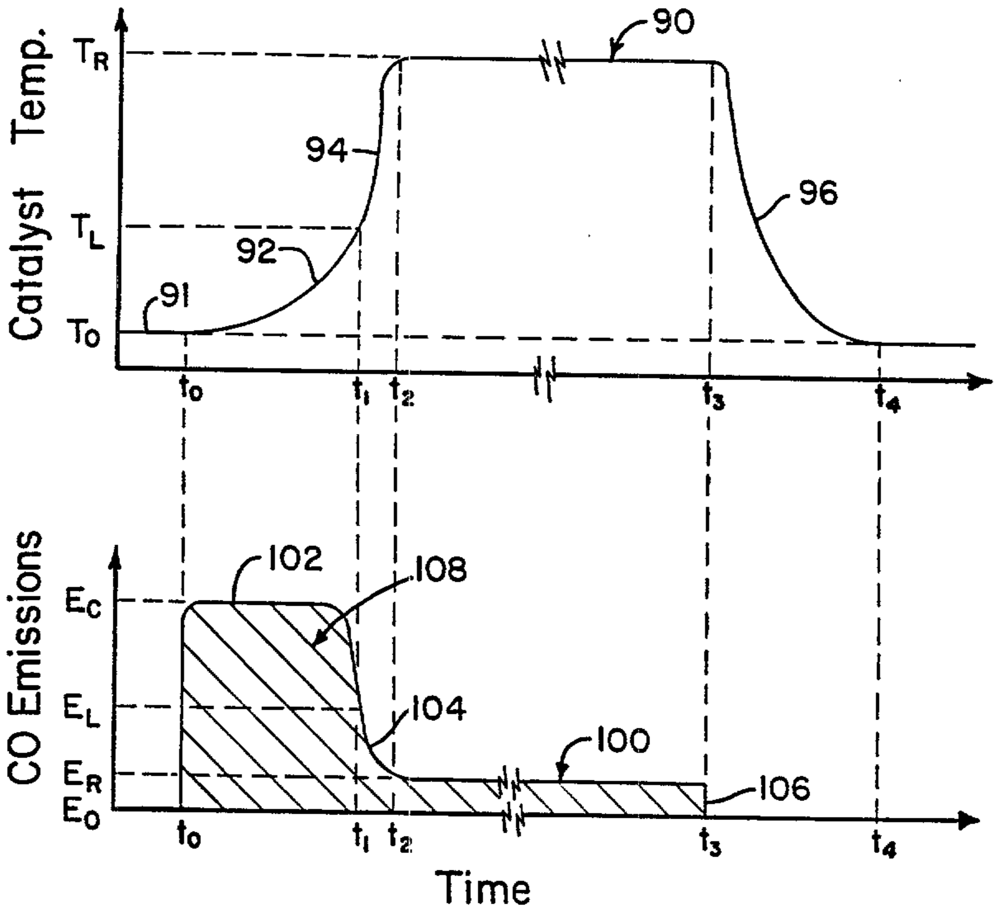
FIG. 3 (Prior Art)
