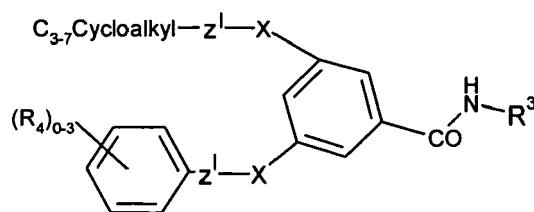
Formula (IIc)
