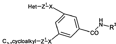
Formula (IIg)
