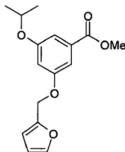
Compound (c)
