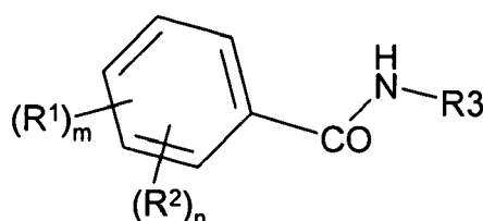
Formula (Id)
