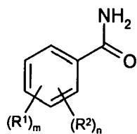
Formula (III)f)
