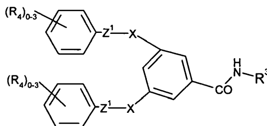
Formula (II)
