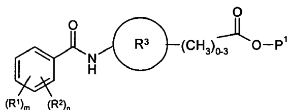
Formula (IIc)
