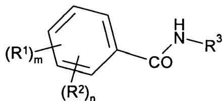
Formula (Ia)
