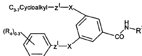
Formula (IIc)
