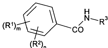
Formula (Ic)
