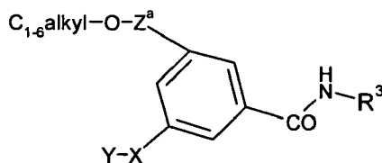
Formula (IIj)
