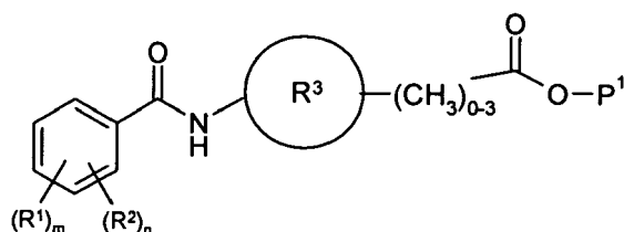
Formula (IIIc)
