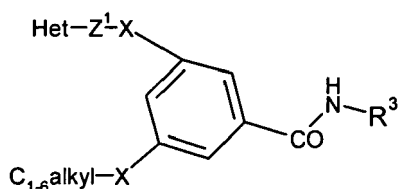
Formula (IIf)
