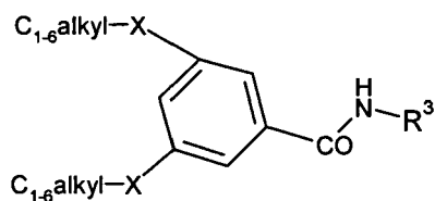
Formula (IId)
