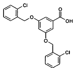
Compound (b)
