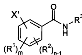
Formula (IIIe)
