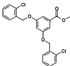
Compound (a)
