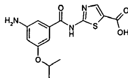
Compound (k)
