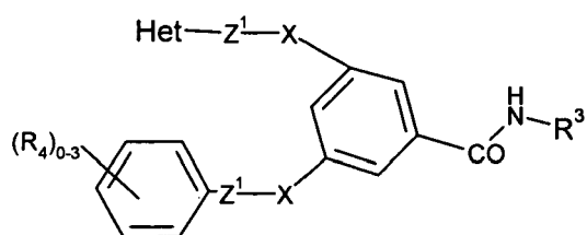
Formula (IIa)
