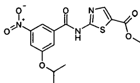
Compound (g)
