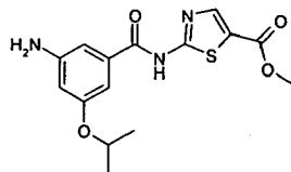
Compound (h)
