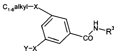
Formula (IIh)
