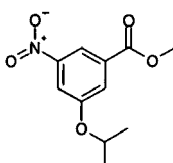
Compound (e)
