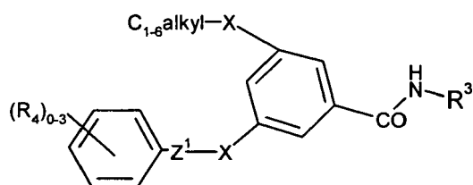
Formula (IIb)
