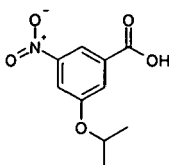
Compound (f)
