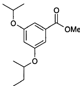
Compound (b)
