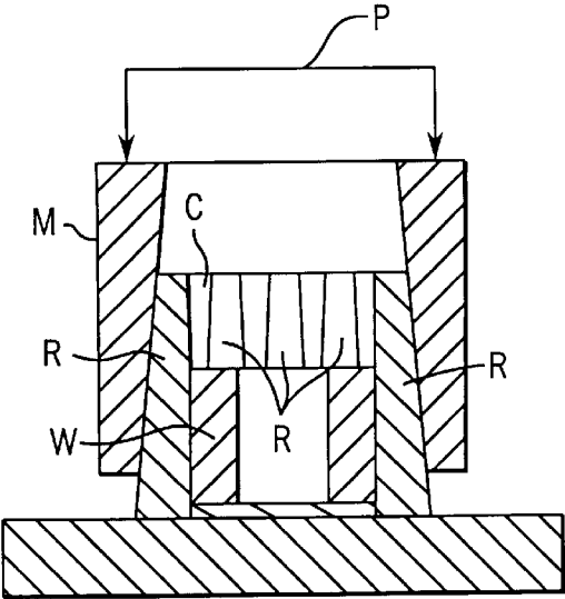
FIG. 2C PRIOR ART
