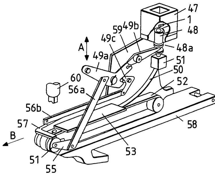
FIG. 32 PRIOR ART
