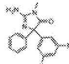
Compound 1B
