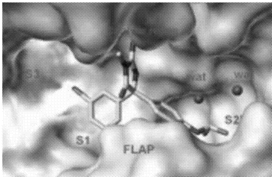
Compound 1A
