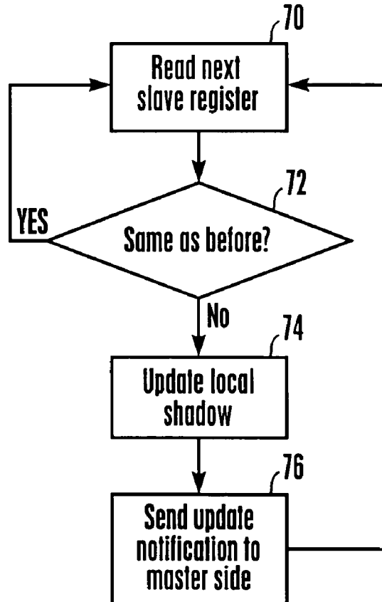
Figure 4 read preparation logic
