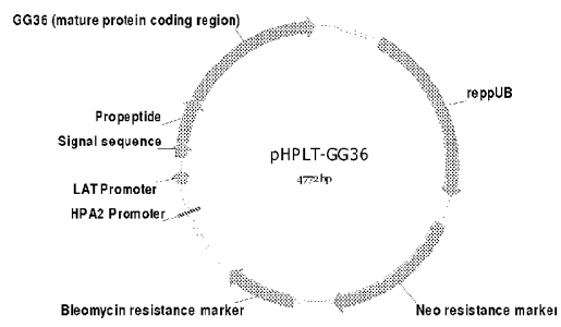
FIGURE 2 - pHPLT-GG36 Expression Plasmid
