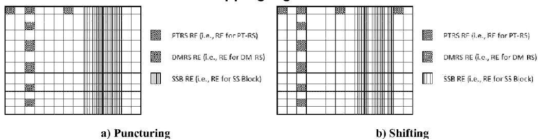
Figure 4. Examples of PTRS collision with SSB with PTRS time density 1/4.
