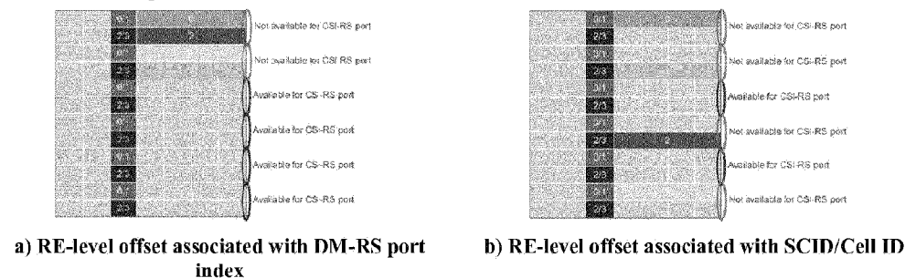
Figure 1. Example of PTRS fixed and configurable mapping and the available CSI-RS ports.
