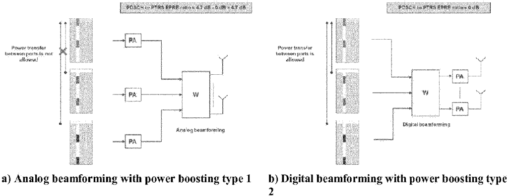
Figure 2. Example of power boosting type 1 and 2 for a transmission with 1 PTRS port, 3 DMRS ports and 3 PDSCH layers.
