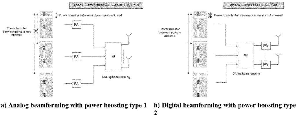
Figure 3. Example of power boosting type 1 and 2 for a transmission with 2 PTRS ports, 3 DMRS ports and 3 PDSCH layers.
