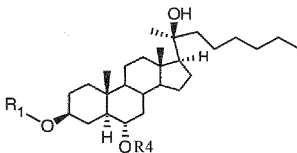
(Formula V),
