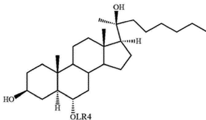
(Formula IX),
