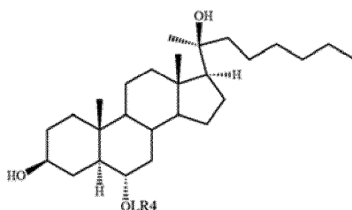
(Formula IX);
