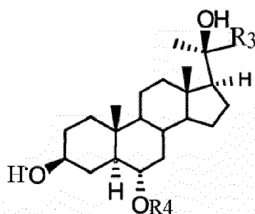
(Formula IVa).
