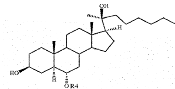
(Formula VI),
