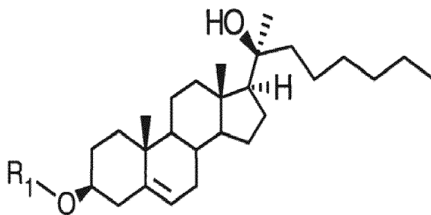
(Formula IIIa).
