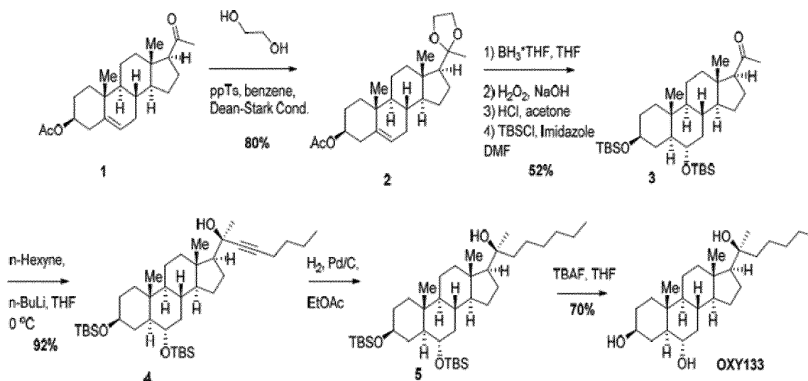
Scheme 3
