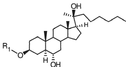
(Formula Va).
