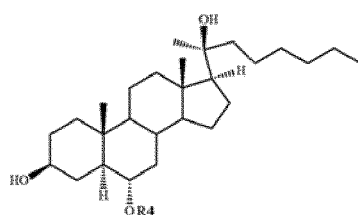
(Formula VI),
