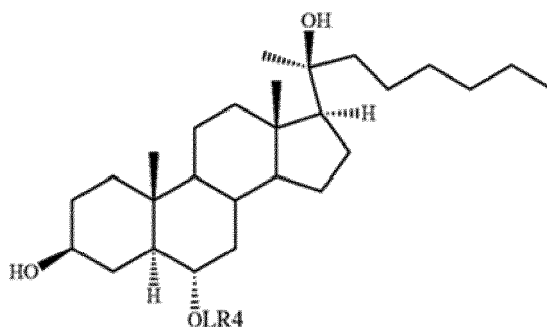
(Formula IX)
