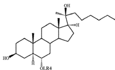
(Formula IX);
