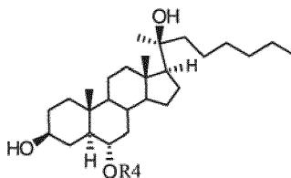
(Formula VI),
