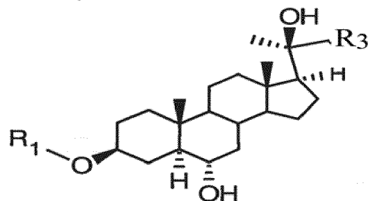
(Formula IV).
