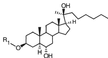
(Formula Va);
