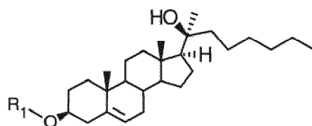
(Formula IIIa);
