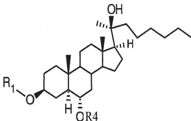
(Formula V),
