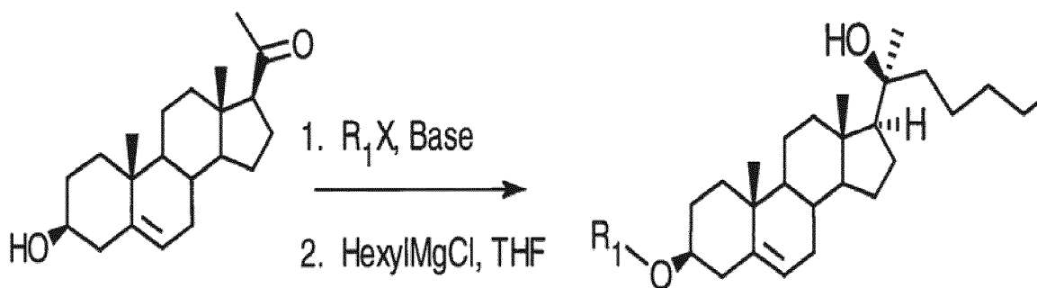
Formula I
