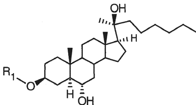
(Formula Va).
