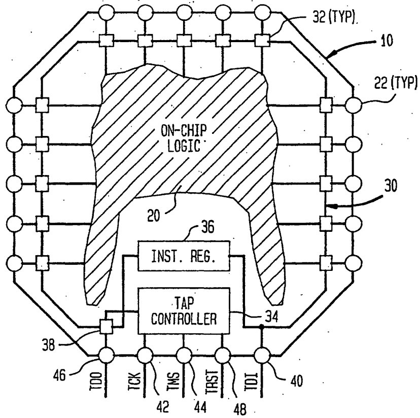
FIG. 1 (PRIOR ART)
