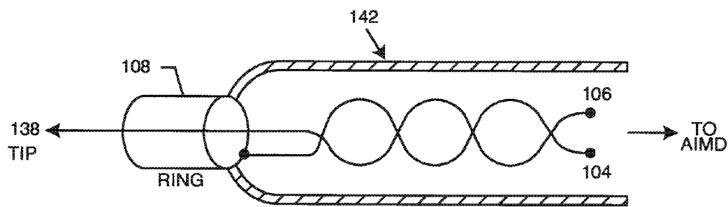
FIG. 22 PRIOR ART
