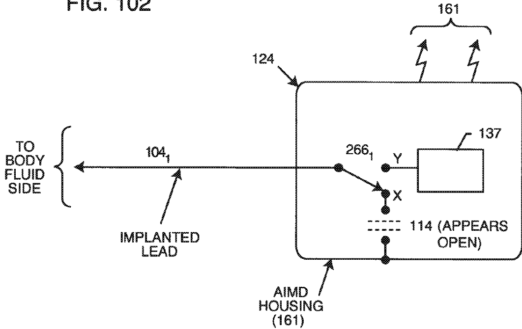
MRI GRADIENT (LOW) FREQUENCY MODEL
