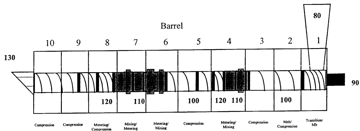
Schematic Diagram of ZSK-30 Extruder Screws and Barrels
