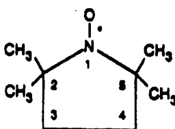
PROXYL (2,2,5,5-Tetramethyl-1-pyrrolidinyl-oxy) (2,2,5,5-Tetramethylpyrrolidine-N-oxy)
