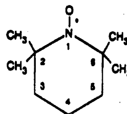
TEMPO (2,2,6,6-Tetramethyl-1-piperidinyl-oxy) (2,2,6,6-Tetramethylpiperidine-N-oxy)
