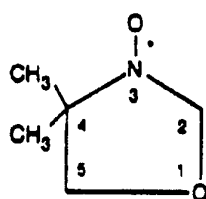
DOXYL (4,4-Dimethyl-3-oxazolinyl-oxy) (4,4-Dimethyloxazolidine-N-oxy)
