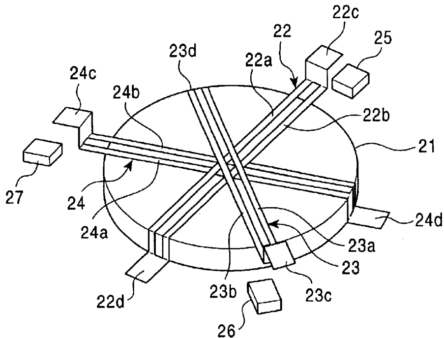
FIG. 8 PRIOR ART
