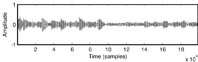
FIG. 10c c) Signal modified with DRC gain
