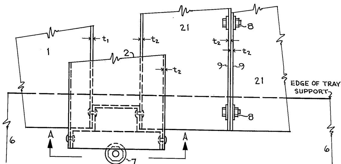
PLAN VIEW FIG. 3
