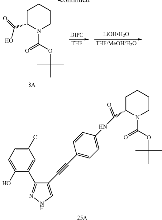
2(S)-{4-[3-(5-Chloro-2-hydroxy-phenyl)-1H-pyrazol-4-ylethynyl]-phenylcarbamoyl}-piperidine-1-carboxylic acid tert-butyl ester (25A)
