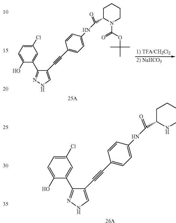
Piperidine-2(S)-carboxylic acid {4-[3-(5-chloro-2-hydroxy-phenyl)-1H-pyrazol-4-ylethynyl]-phenyl}-amide (26A)
