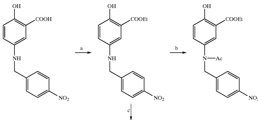
Reaction Scheme 3
