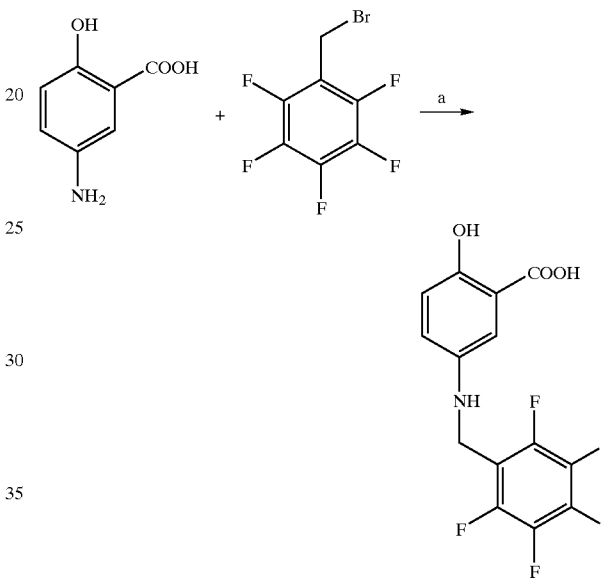
Reaction Scheme 2
