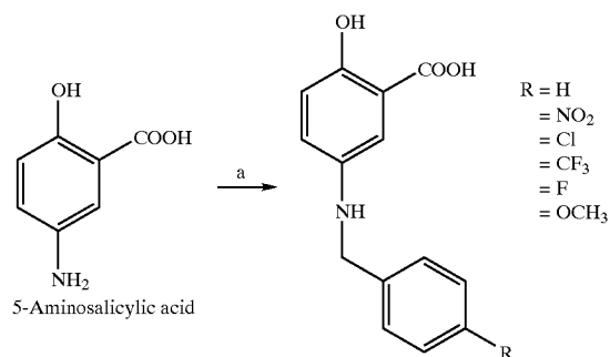
Reaction Scheme 1
