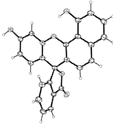
Compound 14a
