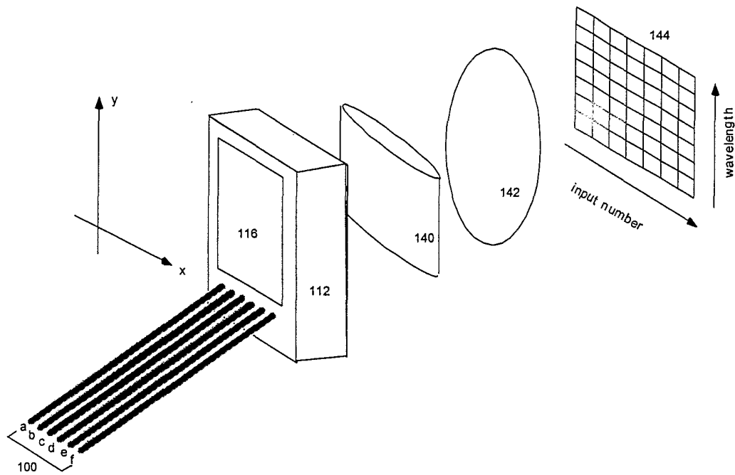
Figure 6. Example embodiment of an Optical Tapped Delay Line (OTDL) channelizer system.
