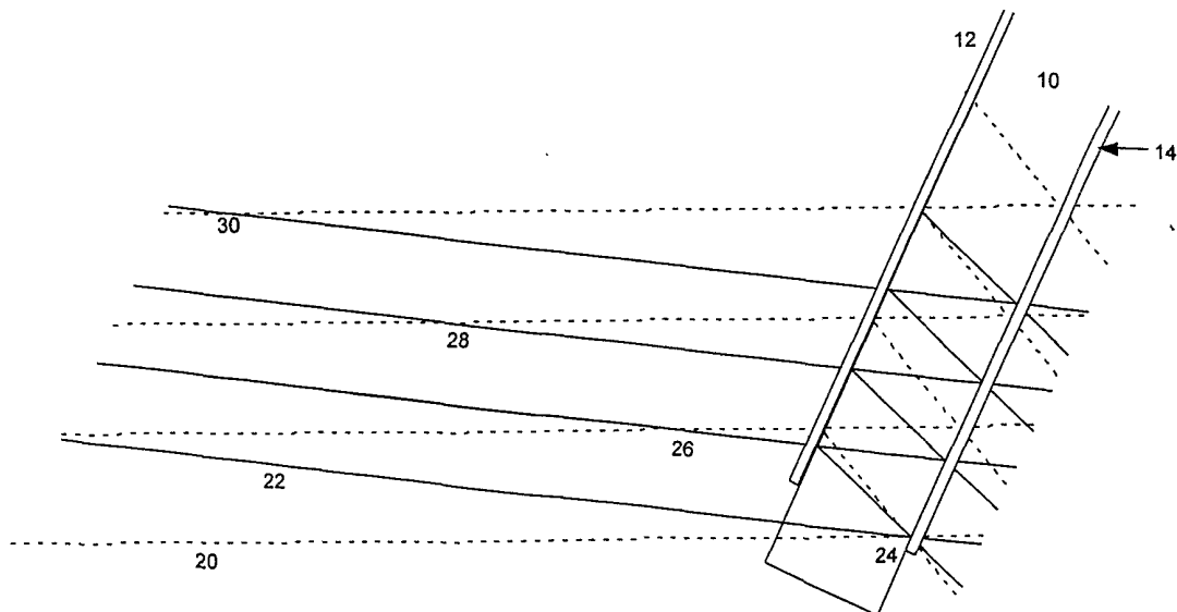
Figure 4. Operation of a prior art VIPA device.
