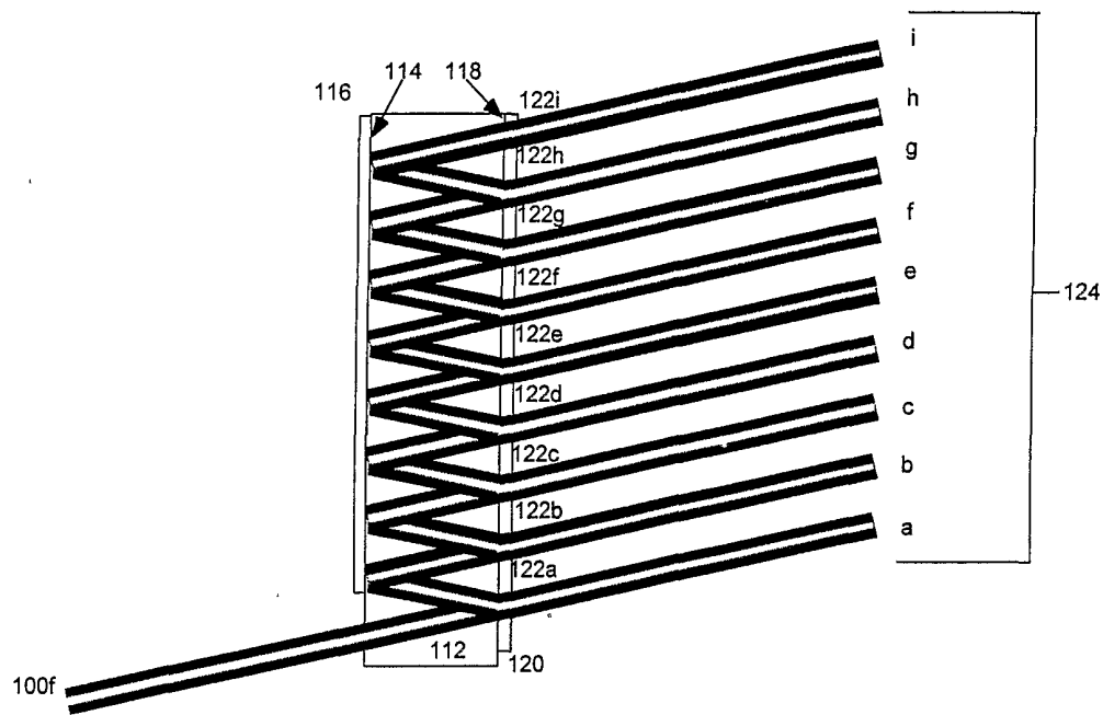
Figure 7. Operational side view of an OTDL device.
