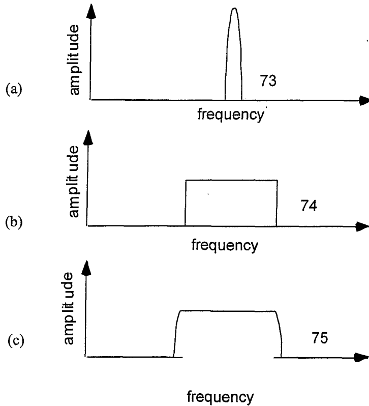
Figure 9. Example channel filter shape for an OTDL channelizer a) Optical spot profile in the output plane of a channelizer. b) Spatial response of a detector element in the output plane. c) Channel filter shape resulting from the convolution of 73 and 74.
