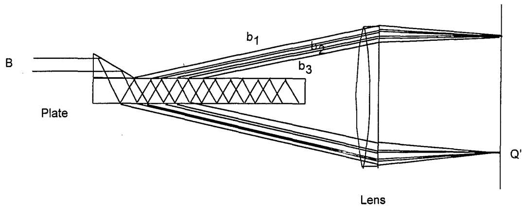
Figure 2. Prior art of a Lummer-Gehrcke interferometer.
