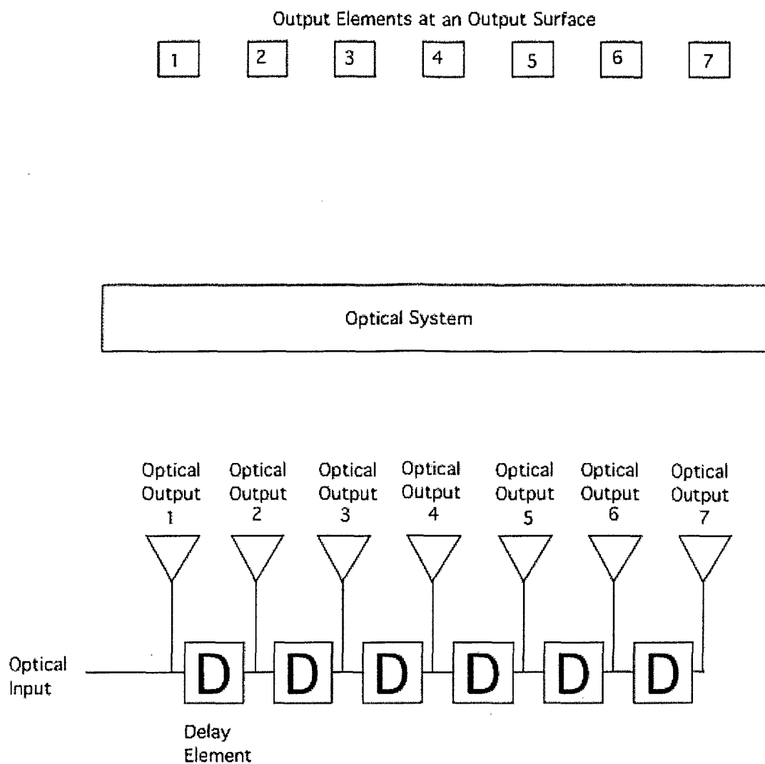
Figure 11. Functional block diagram of an OTDL device including an optical system and output elements at an output surface.
