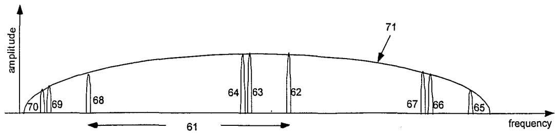
Figure 8. Example optical distribution along the frequency axis of an OTDL channelizer output.
