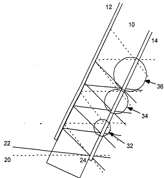
Figure 5. Beam overlap and interference in a VIPA device prior art.
