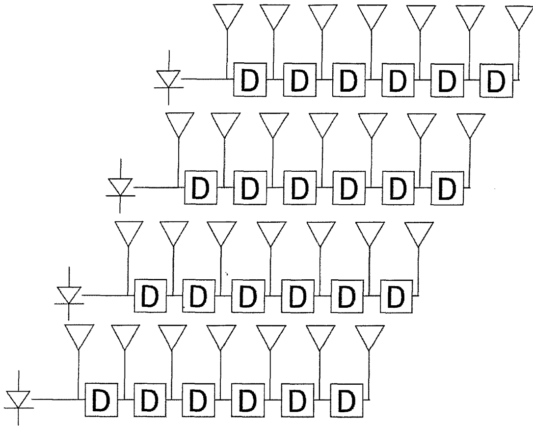
Figure 12. Functional block diagram of an OTDL device shown in a multiple input arrangement.
