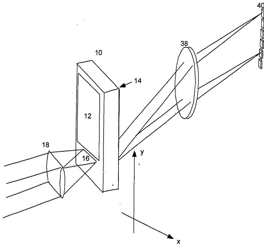
Figure 3. Prior art of a Virtually Imaged Phased Array (VIPA) channelizer.
