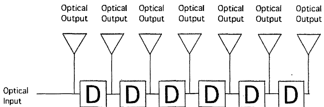
Figure 10. Functional block diagram of an OTDL device shown in a single input arrangement.
