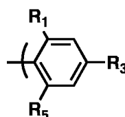
(IIc)
