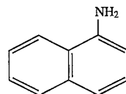
a-naphthylamine
