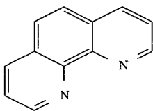
1,10-phenanthroline
