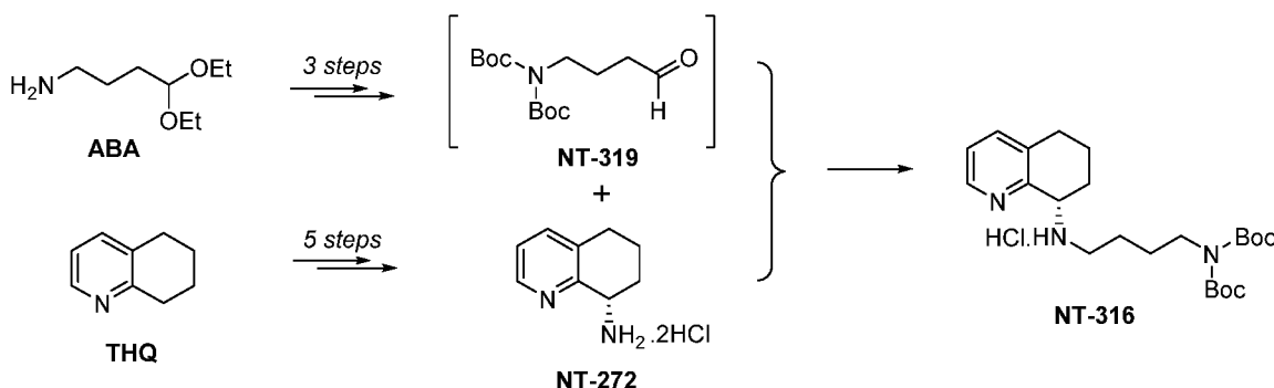
Scheme 7: Early steps in the synthesis of X4P-001.
