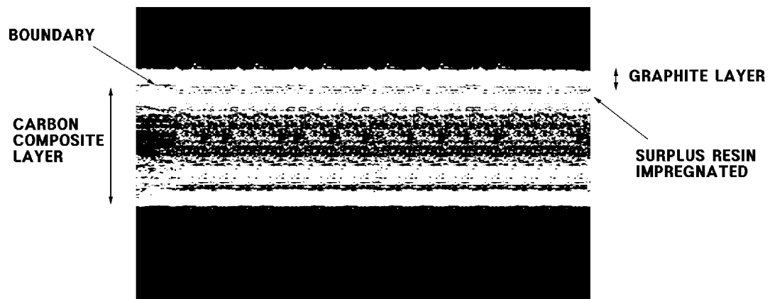
CROSS SECTION VIEW OF THE COMPOSITE+GF PLATE
