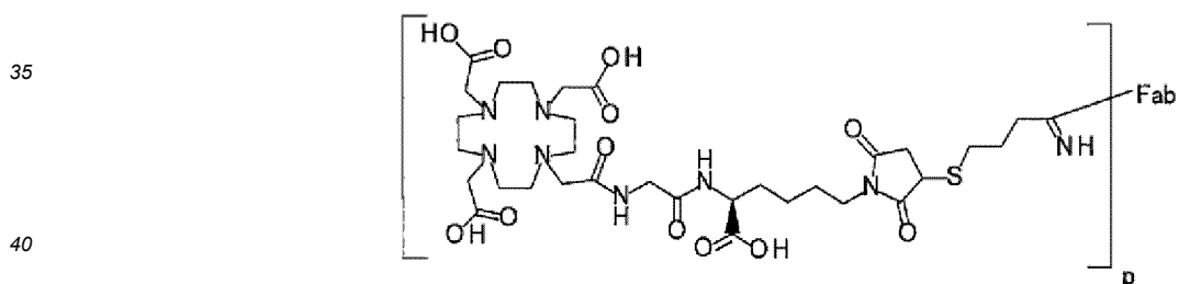
[Chemical Formula 3]
