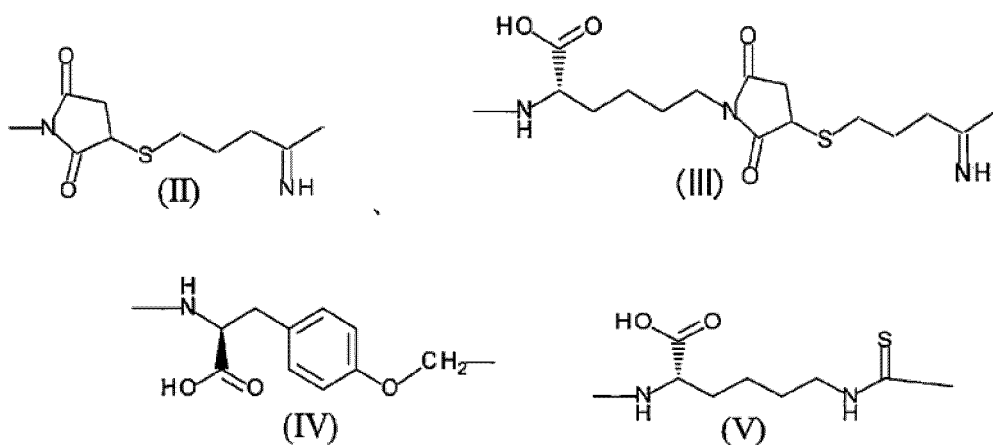
[Chemical Formula 1]
