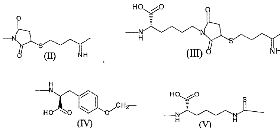
[Chemical Formula 1]
