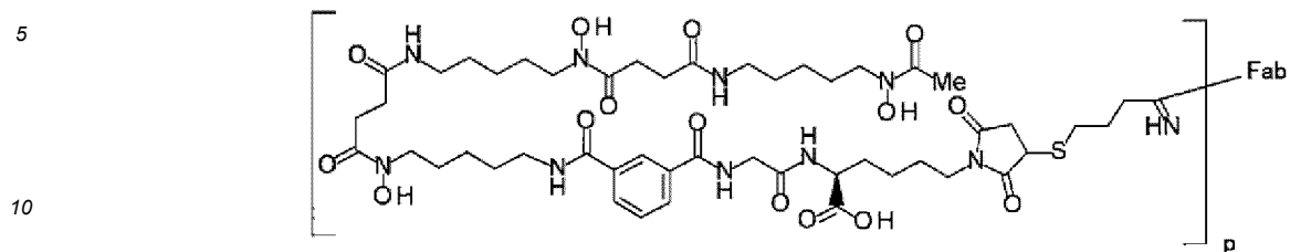
[Chemical Formula 2]
