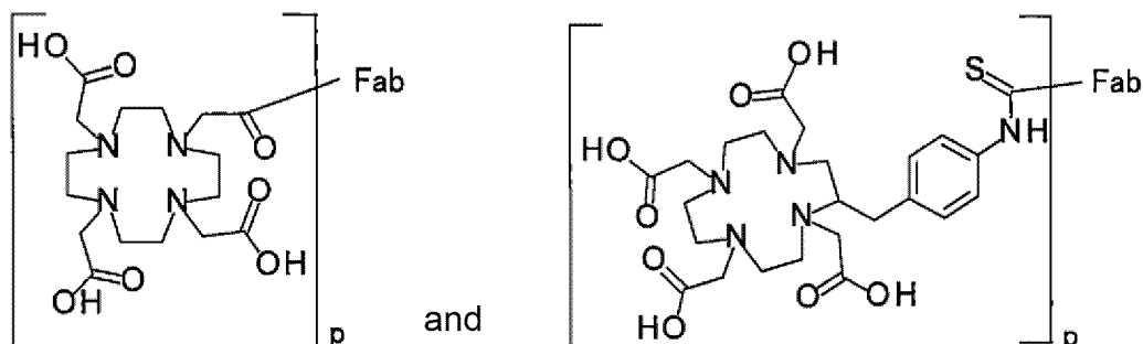
[Chemical Formula 4]
