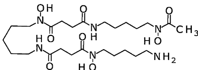
[Chemical Formula 5]
