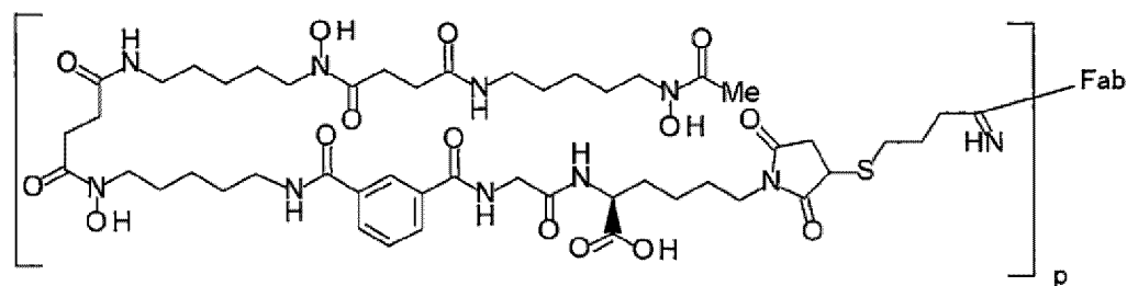
[Chemical Formula 2]
