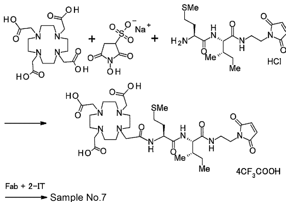
[Chemical Formula 16]
