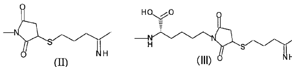
[Chemical Formula 7]
