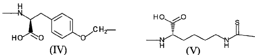
[Chemical Formula 8]
