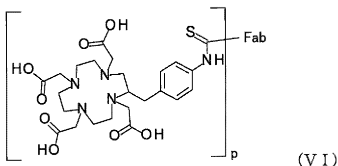
[Chemical Formula 9]
