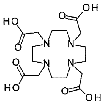
[Chemical Formula 6]
