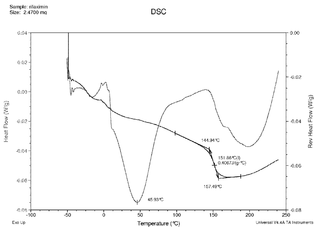
Figure 37. Modulate DSC thermograms for 25:75 (w/w) Rifaximin/HPMC-P dispersion
