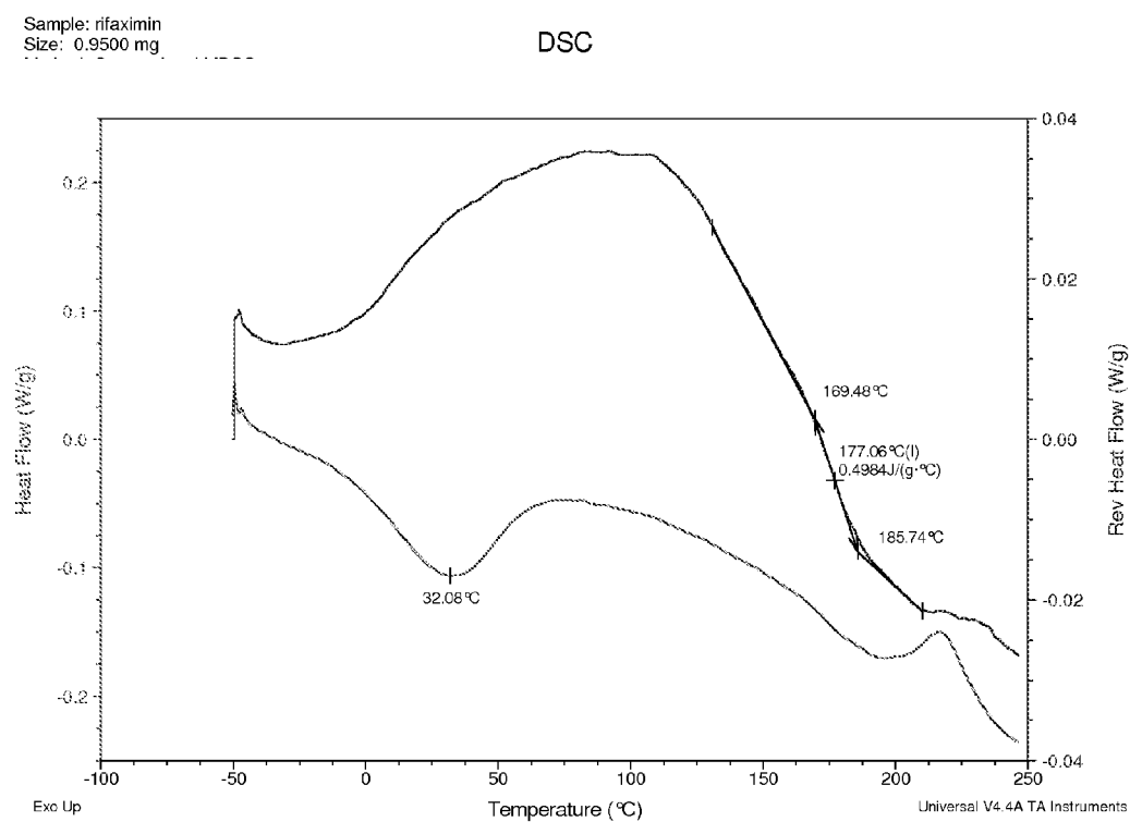
Figure 28. mDSC thergram for 75:25 (w/w) Rifaximin/HPMC-AS HG dispersion stressed at 40 °C/75% RH for 7 d
