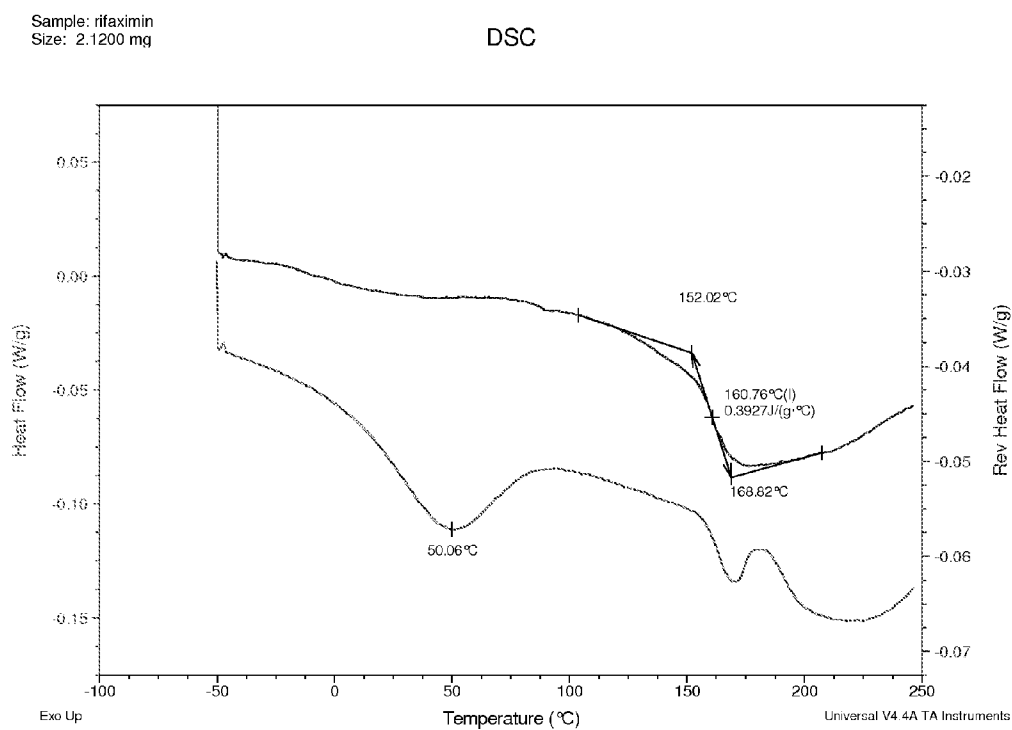
Figure 9. mDSC thermogram for 50:50 (w/w) Rifaximin/HPMC-P dispersion obtained from methanol by spray drying
