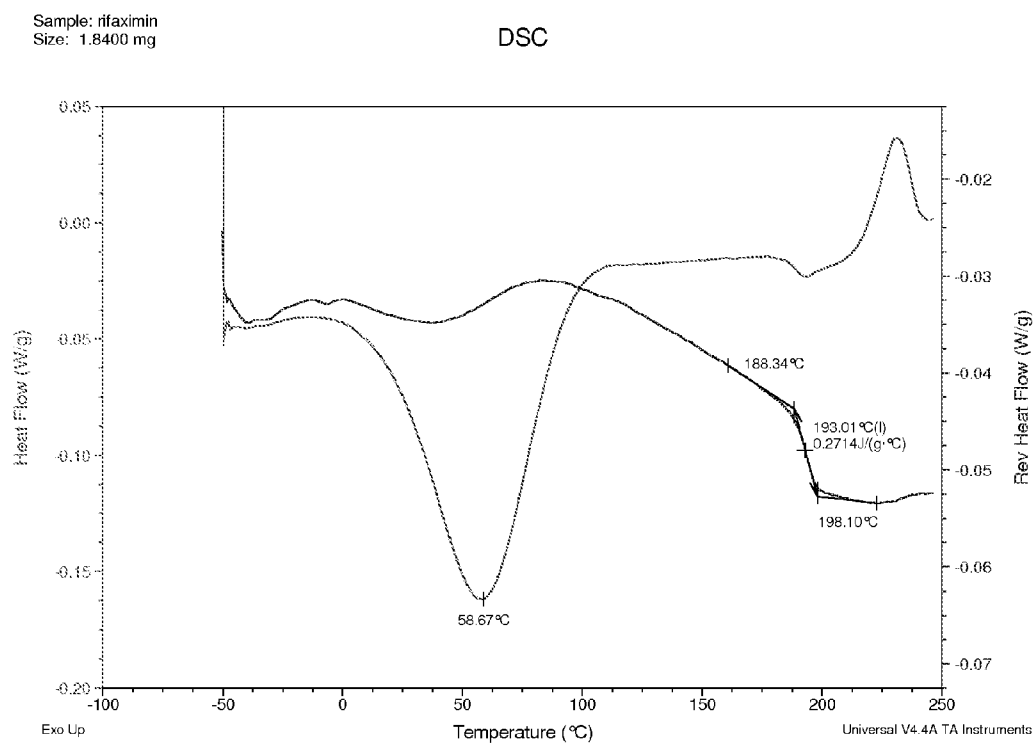
Figure 4. mDSC thermogram for 50:50 (w/w) Rifaximin/PVP K-90 dispersion obtained from methanol by spray drying
