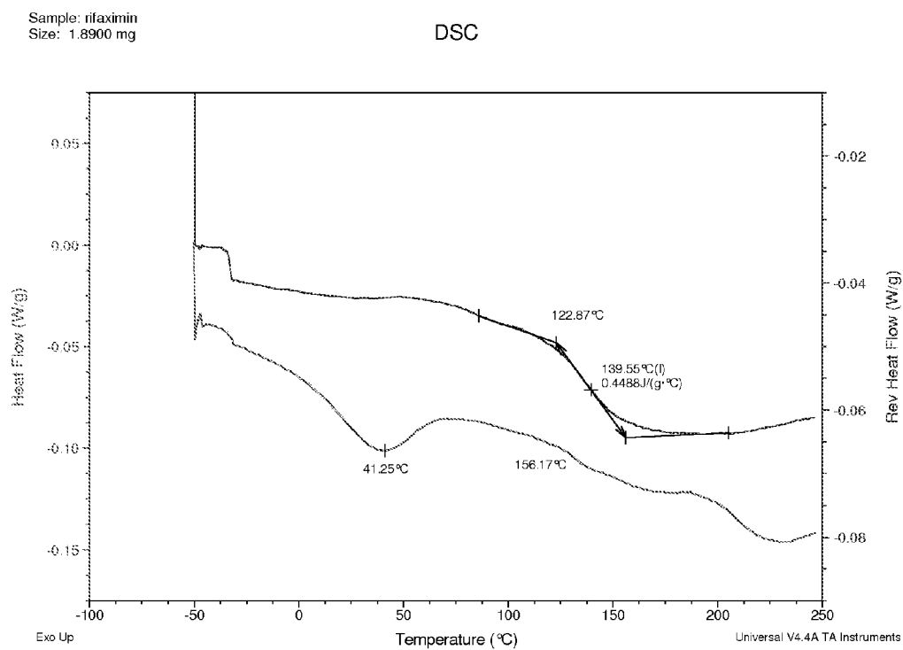
Figure 18. mDSC thermogram for 25:75 (w/w) Rifaximin/HPMC-AS MG dispersion obtained from methanol by spray drying
