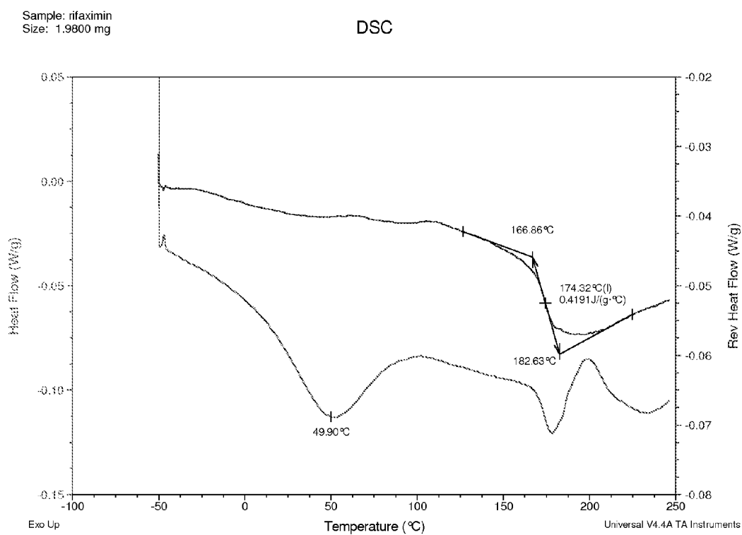
Figure 10. mDSC thermogram for 75:25 (w/w) Rifaximin/HPMC-P dispersion obtained from methanol by spray drying
