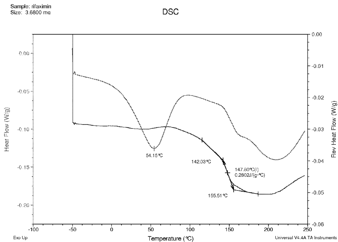
Figure 27. mDSC thergram for 25:75 (w/w) Rifaximin/HPMC-P dispersion stressed at 40 °C/75% RH for 7 d
