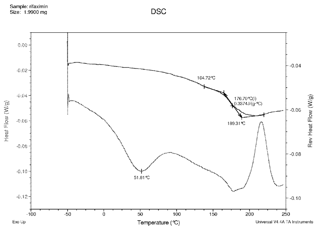
Figure 20. mDSC thermogram for 75:25 (w/w) Rifaximin/HPMC-AS MG dispersion obtained from methanol by spray drying
