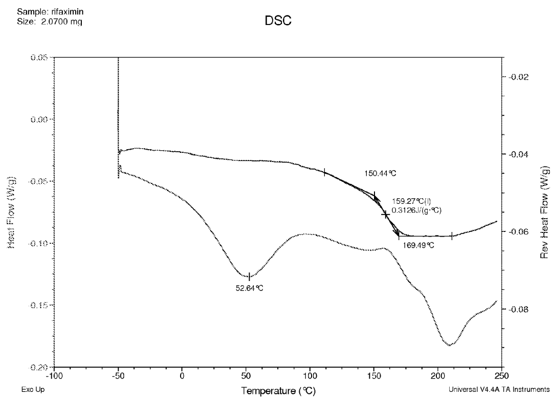
Figure 24. mDSC thermogram for 50:50 (w/w) Rifaximin/Eudragit L100-55 dispersion obtained from methanol by spray drying
