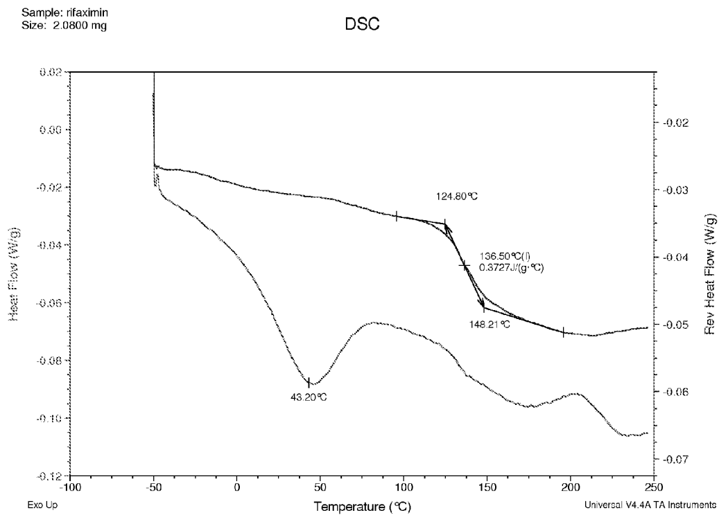
Figure 13. mDSC thermogram for 25:75 (w/w) Rifaximin/HPMC-AS HG dispersion obtained from methanol by spray drying
