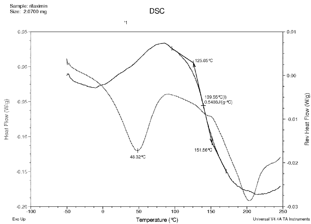
Figure 30. mDSC thergram for 25:75 (w/w) Rifaximin/Eudragit L100-55 dispersion stressed at 40 °C/75% RH for 7 d
