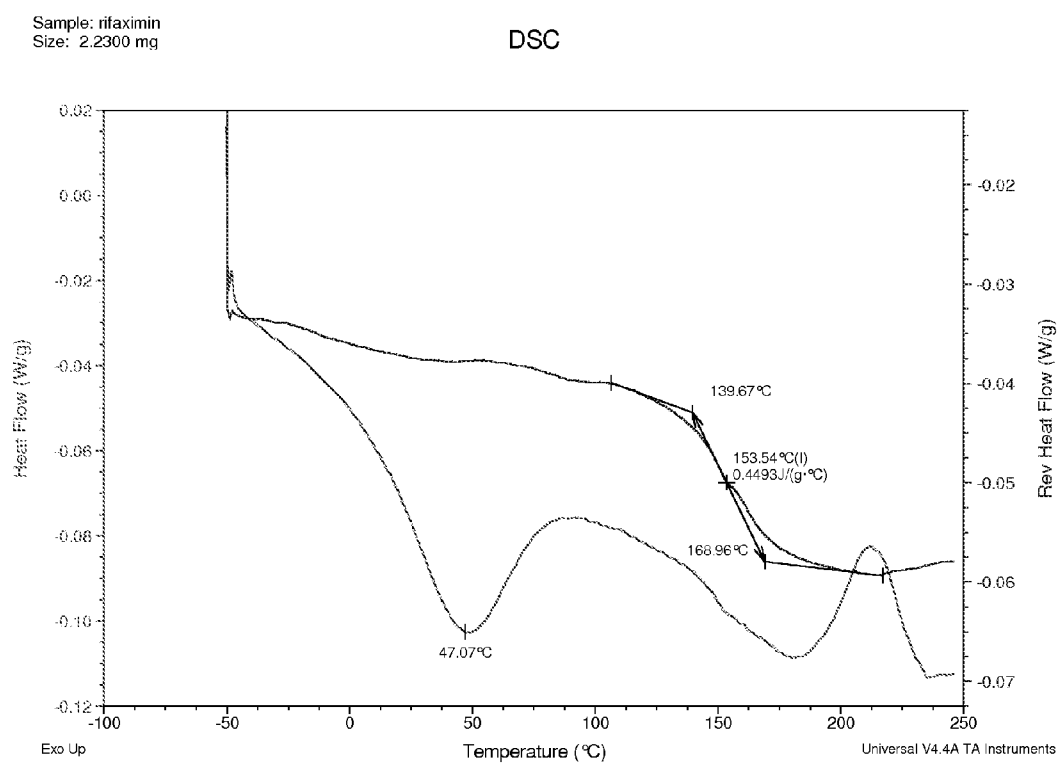
Figure 14. mDSC thermogram for 50:50 (w/w) Rifaximin/HPMC-AS HG dispersion obtained from methanol by spray drying
