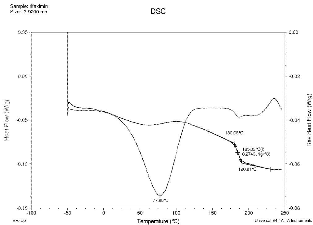
Figure 3. mDSC thermogram for 25:75 (w/w) Rifaximin/PVP K-90 dispersion obtained from methanol by spray drying
