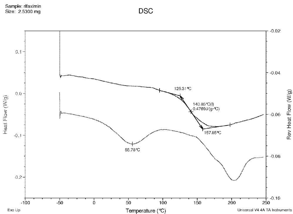
Figure 23. mDSC thermogram for 25:75 (w/w) Rifaximin/Eudragit L100-55 dispersion obtained from methanol by spray drying
