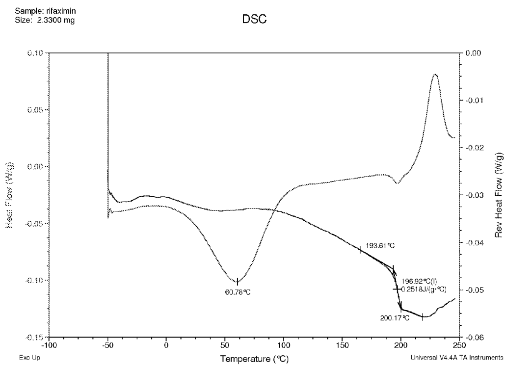
Figure 5. mDSC thermogram for 75:25 (w/w) Rifaximin/PVP K-90 dispersion obtained from methanol by spray drying
