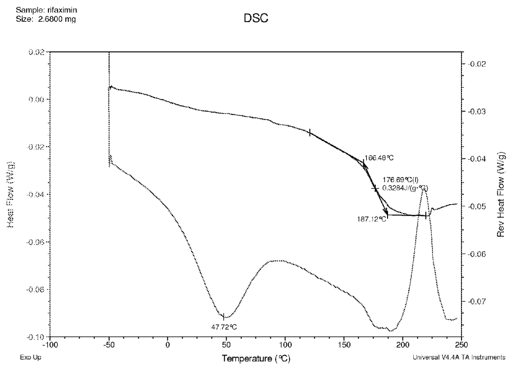
Figure 15. mDSC thermogram for 75:25 (w/w) Rifaximin/HPMC-AS HG dispersion obtained from methanol by spray drying
