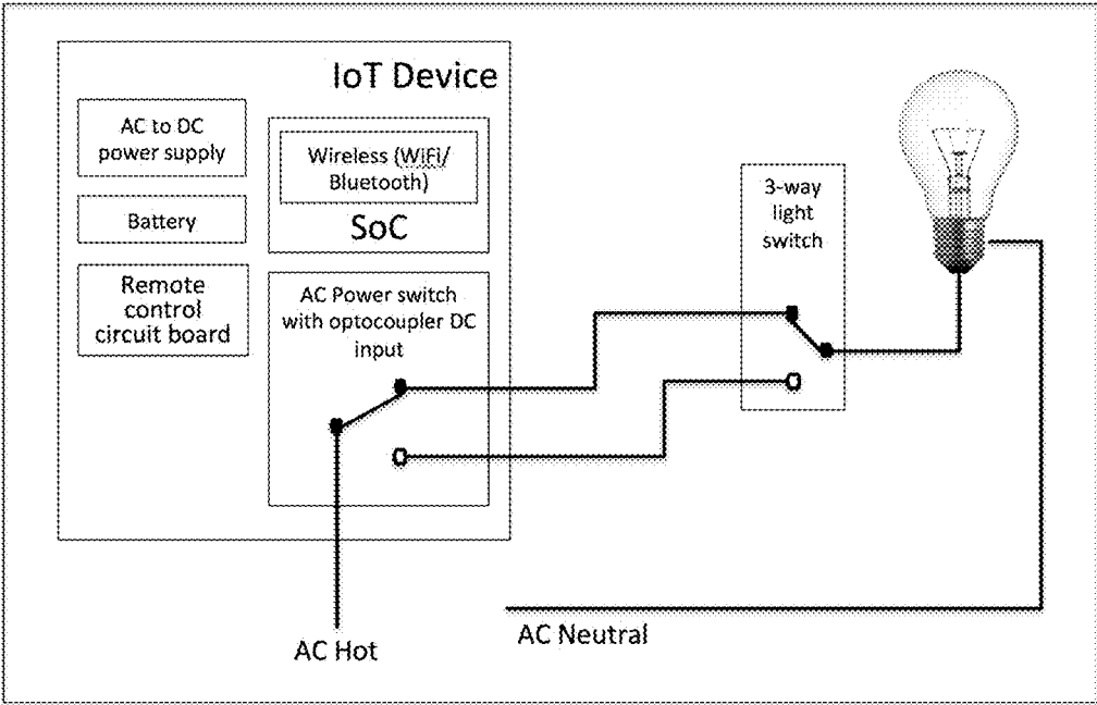
Figure 10 - 1000. 3-Way Light Switch
