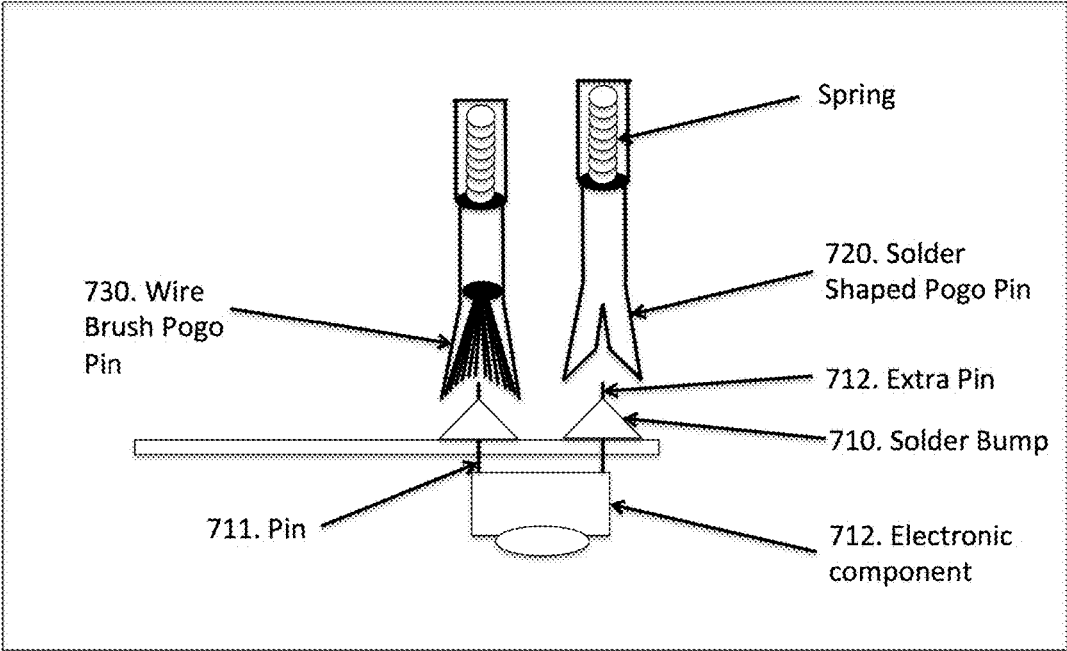
Figure 7 – 700. Solder Shaped and Wire Brush Pogo Pins
