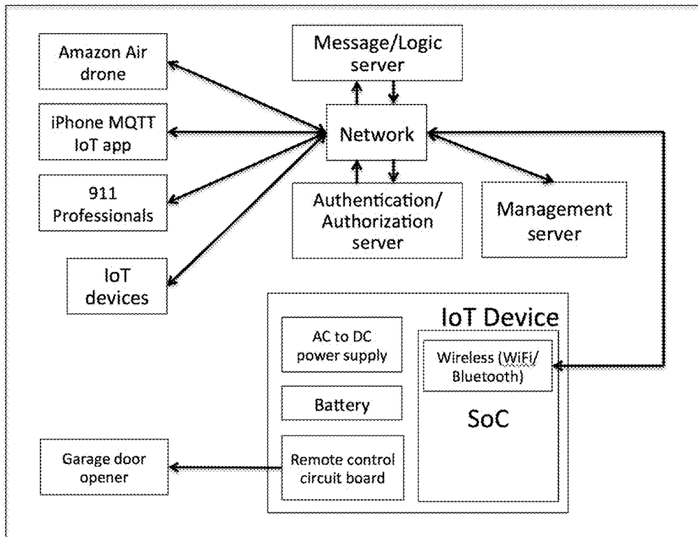
Figure 8 - 800. Flowchart
