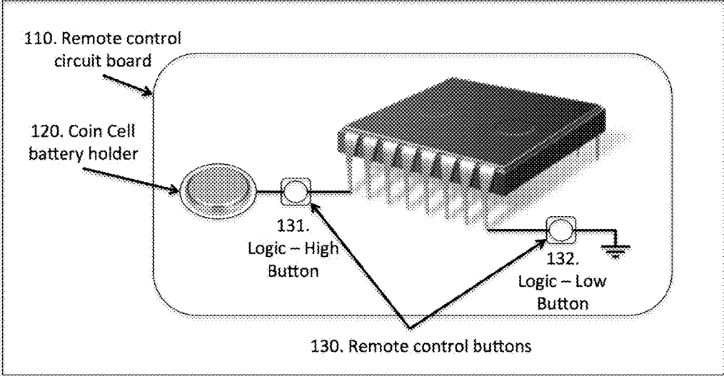
Figure 1 - 100. Garage Remote Control
