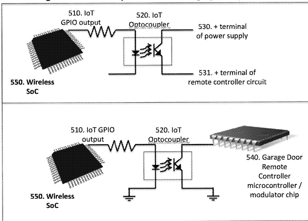
Figure 5 - 500. Examples of Circuit using Optocoupler
