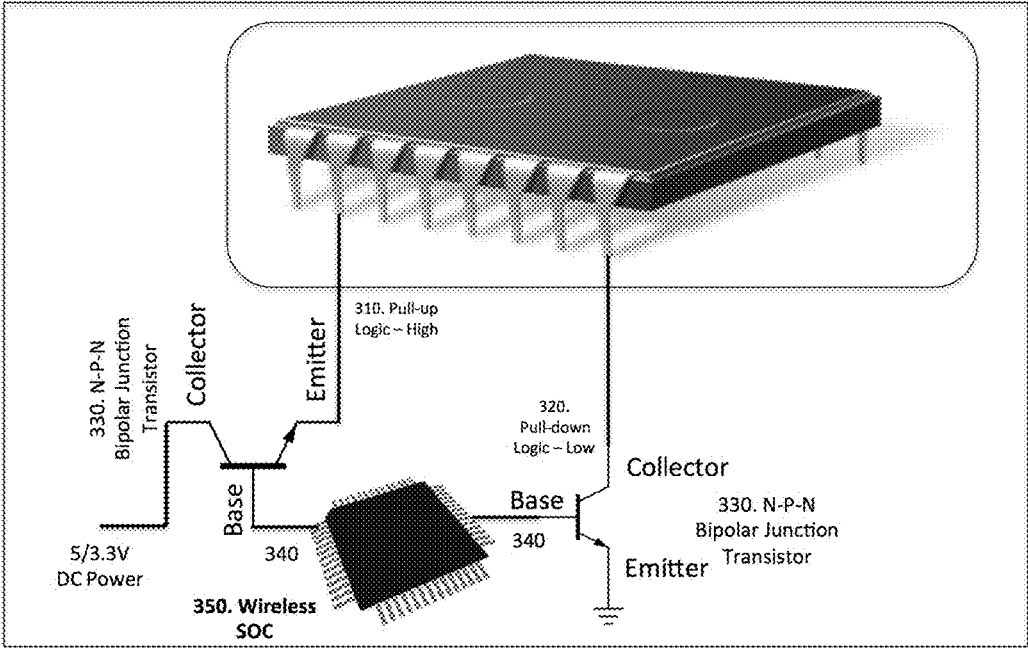
Figure 3 - 300. Coupled with IoT Device using BJT
