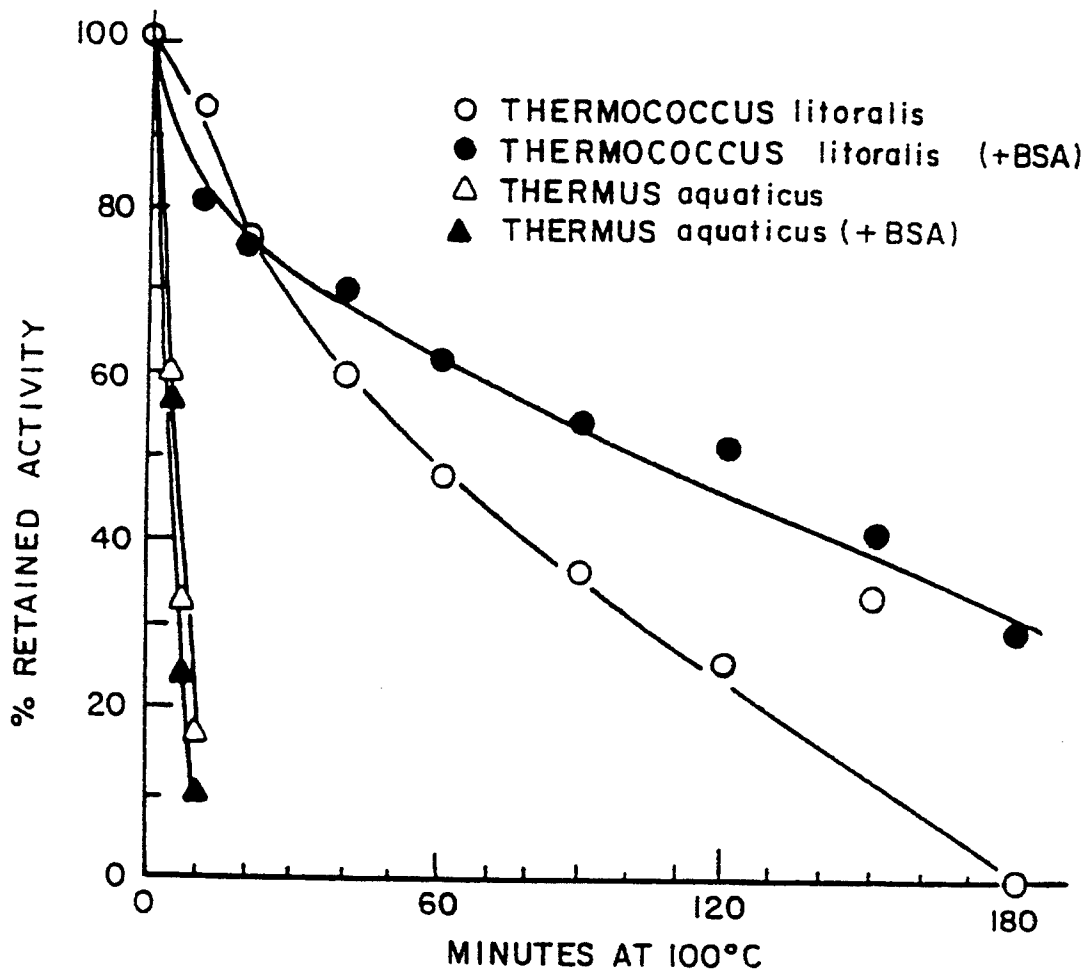
THERMAL STABILITIES OF DNA POLYMERASES
