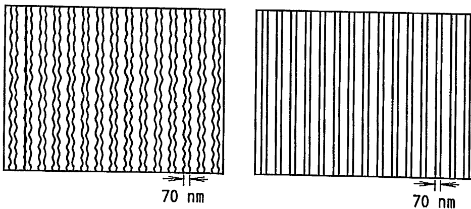
THE 70 nm WIDE AND 100 nm THICK Si GRATINGS ON SOI, BEFORE (a) AND (b) AFTER SELF. THE SEVER ZIG-ZAG EDGES BECOME STRAIGHT AND SMOOTH AFTER SELF.
