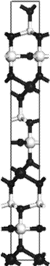
Crystal structure
