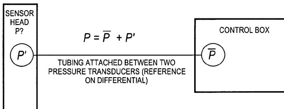
BLOCK DIAGRAM OF A PRESSURE MEASUREMENT SCHEME
