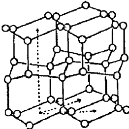
HEXAGONAL DIAMOND
