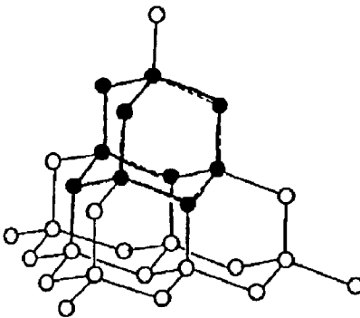
DIAMOND
