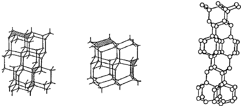
CUBIC DIAMOND
