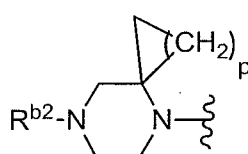
Formula Fb 4a ,
