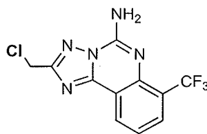
(Compound 8H )
