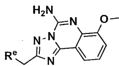
CC4a , or a salt thereof,
