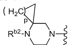
Formula Fb 3a ,
