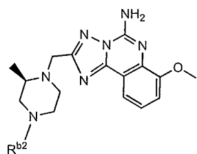
CC6, or a salt thereof,
