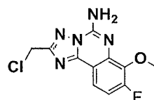
(Compound 8e )
