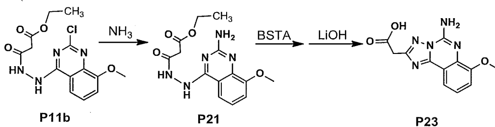
Scheme PV
