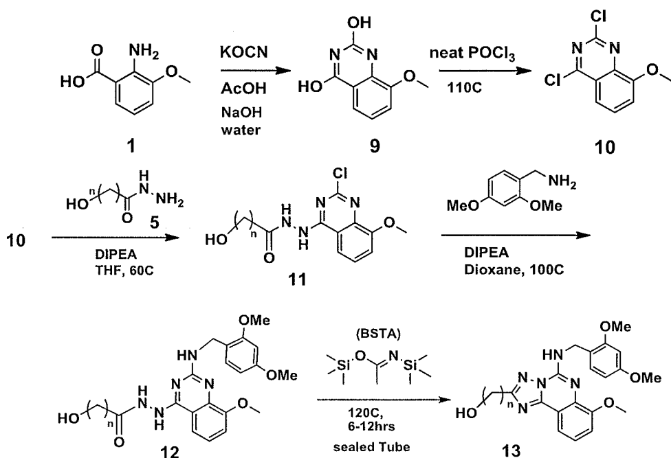
Scheme BII
