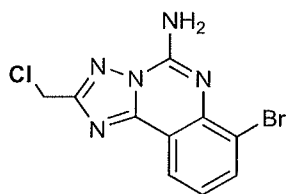
(Compound 8G )
