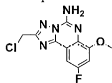
(Compound 8d )
