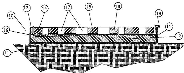
SCHEMATIC OF PREFERRED EMBODIMENT OF ENGINEERED LANDSCAPE/FLOWER PANEL SHOWING CROSS SECTION VIEW AND ALL COMPONENTS.
