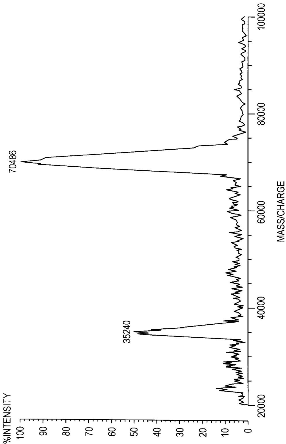
MALDI MASS SPECTRUM OF BSA-DIGOXIGENIN COMPLEX
