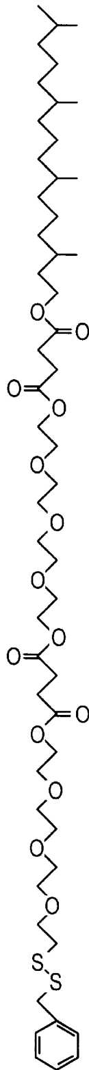
LINKER LIPID A
