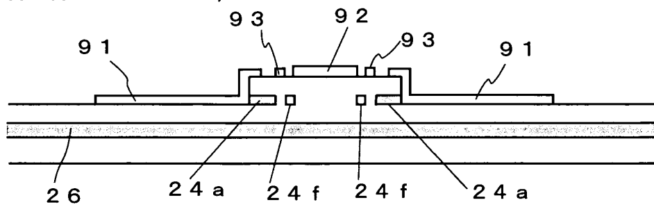
( b ) ( X - X' Cross Section )
