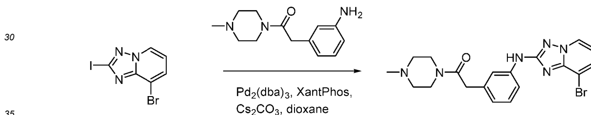
2-[3-([8-bromo-[1,2,4]triazolo[1,5-a]pyridin-2-yl]amino)phenyl]-1-(4-methylpiperazin-1-yl)ethan-1-one
