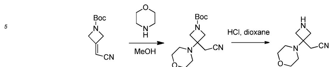
2-[3-(morpholin-4-yl)azetidin-3-yl]acetonitrile
