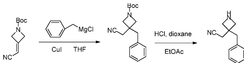
2-(3-benzylazetidin-3-yl)acetonitrile
