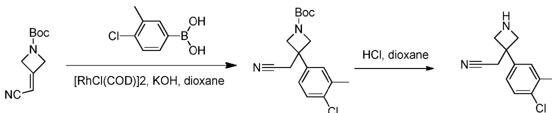
2-[3-(4-chloro-3-methylphenyl)azetidin-3-yl]acetonitrile
