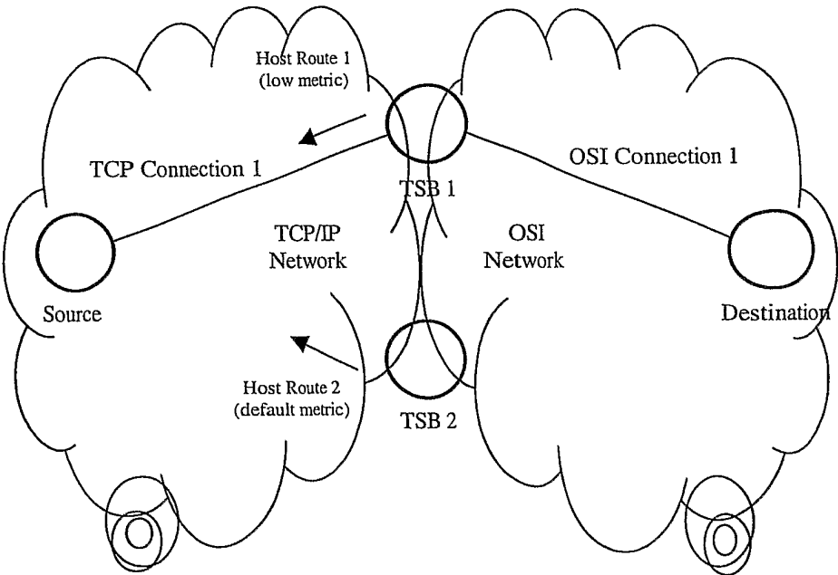
Fig. 10. State 6 (secondary path established).
