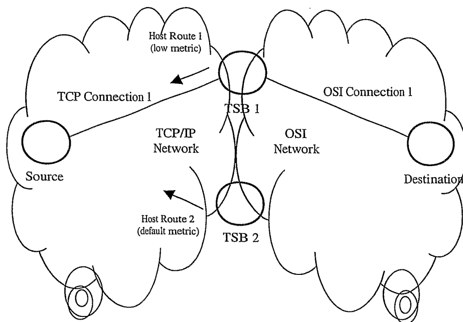
Fig. 6. State 2 (TCP and OSI connections established – both routes advertised).
