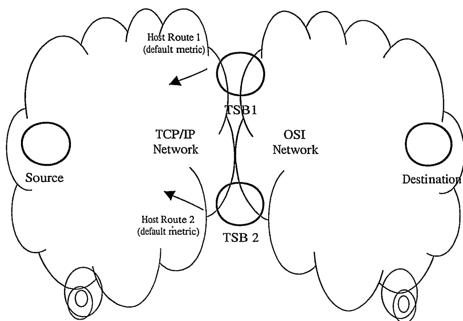
Fig. 5. State 1 (both routes advertised – no connections established).
