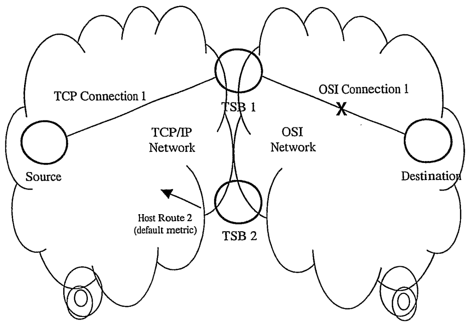
Fig. 7. State 3 (OSI connection fails).
