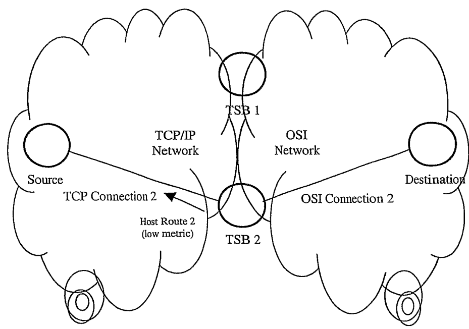
Fig. 8. State 4 (Secondary Path established).
