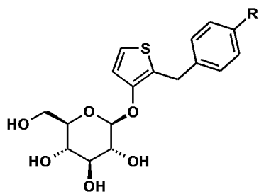
(12) a thiophene derivative of the formula (12)
