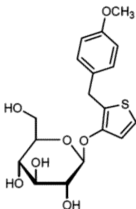
(11) Remogliflozin, represented by formula (11):
