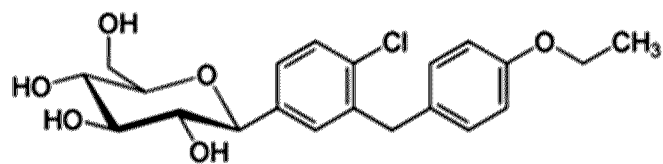
(4) Canagliflozin, represented by formula (4):
