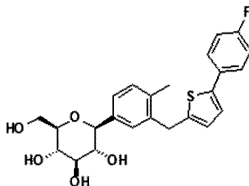
(6) Luseogliflozin, represented by formula (6):
