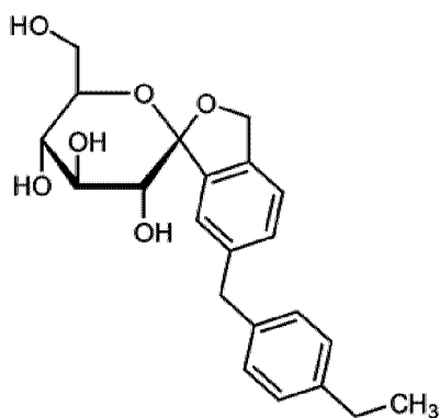
(7) Tofogliflozin, represented by formula (7):
