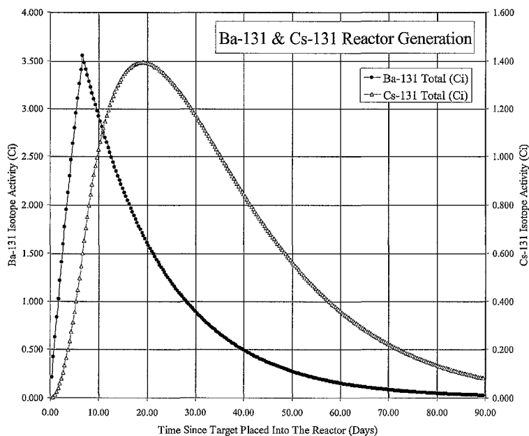
Reactor Generation of Ba-131 and Cs-131 In-Growth
