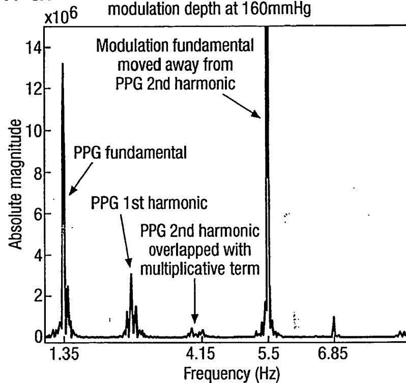
Fig.7e. Optimitised modulation frequency in this particular embodiment
