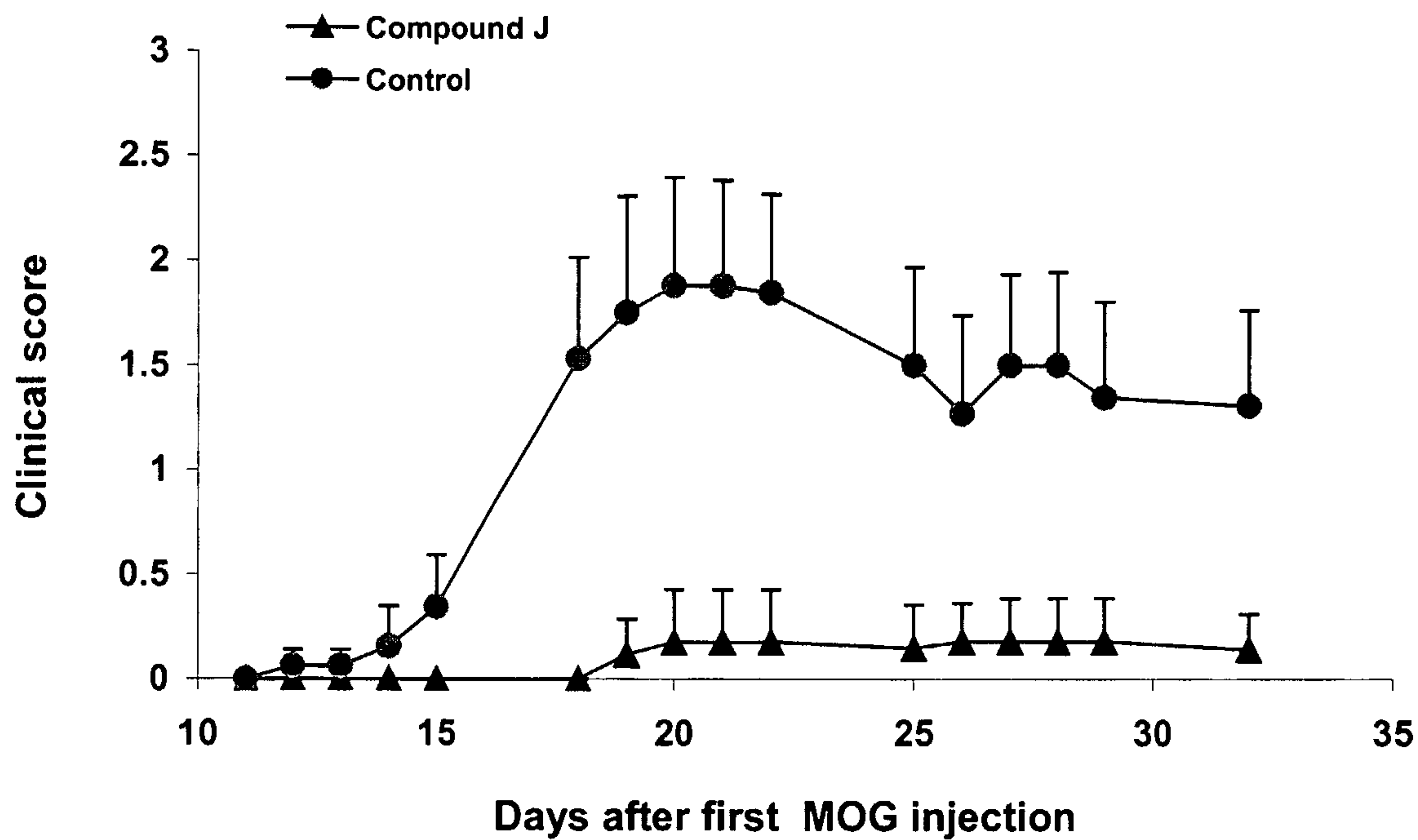
FIG. 7: Compound J treatment (200mg/kg i.p x2, and 300mg/kg in water from day 1) in MOG-induced C3H mice
