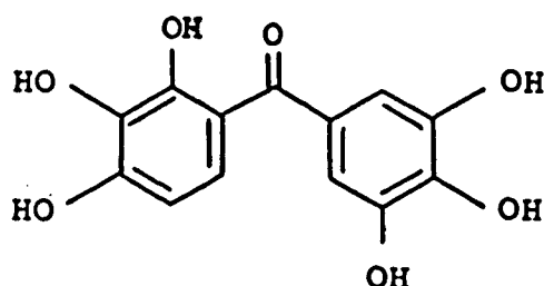
[2,3,4,3',4',5'-Hexahydroxybenzophenone]
