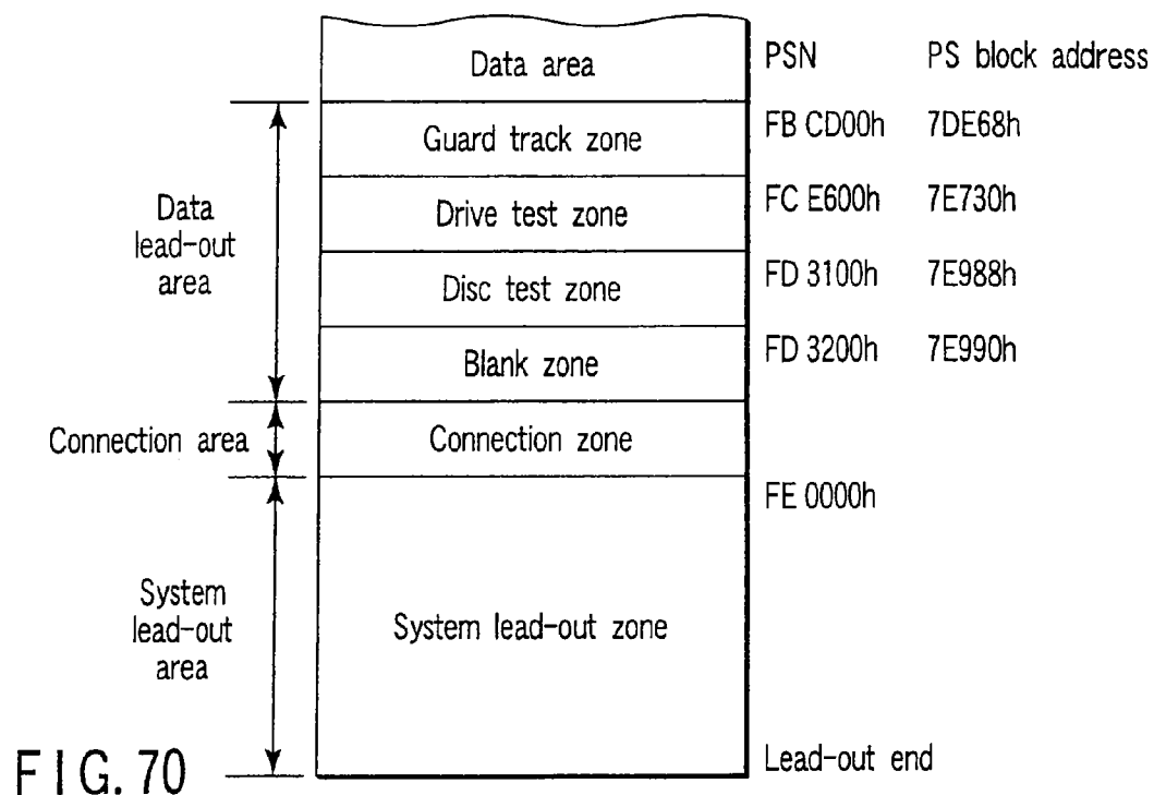
Structure of lead-out area
